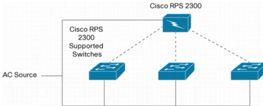
Figure 4. Cisco RPS 2300 Using a Different Circuit from the Connected Network Devices
