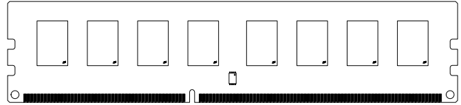
Figure 1: 240-Pin UDIMM (MO-269 R/C-B1)
