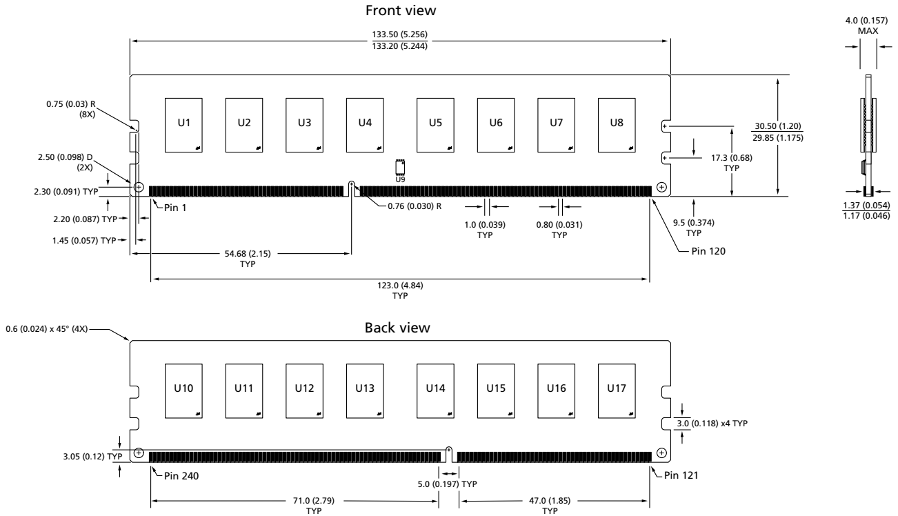
Figure 3: 240-Pin DDR3 UDIMM (R/C-B1)
