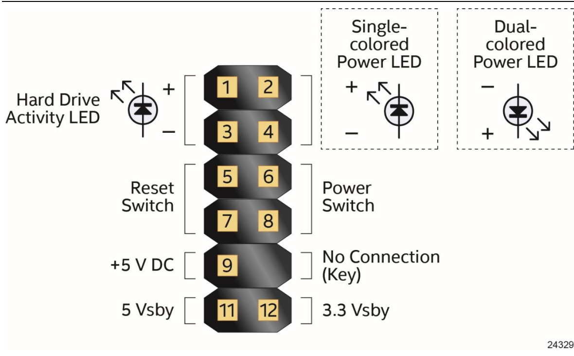
Figure 13. Connection Diagram for Front Panel Header (2.0 mm Pitch)
